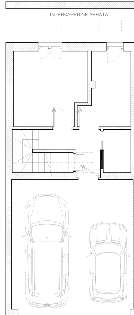
PIANO SEMINTERRATO*
