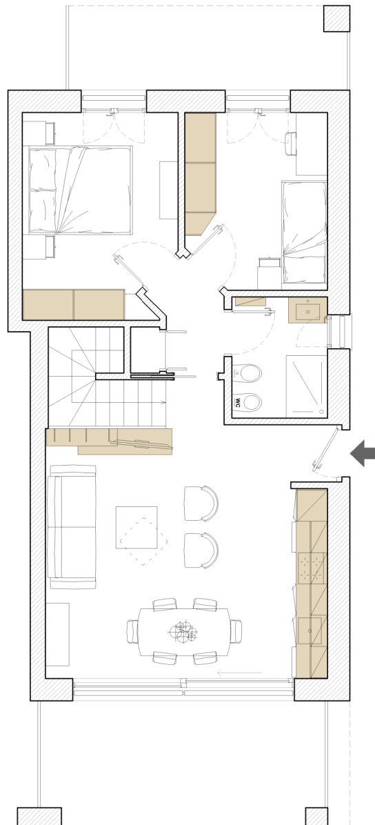
PIANO TERRA
